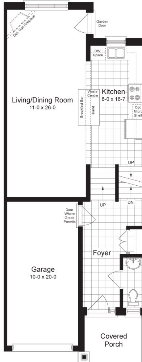
MAIN FLOORPLAN
