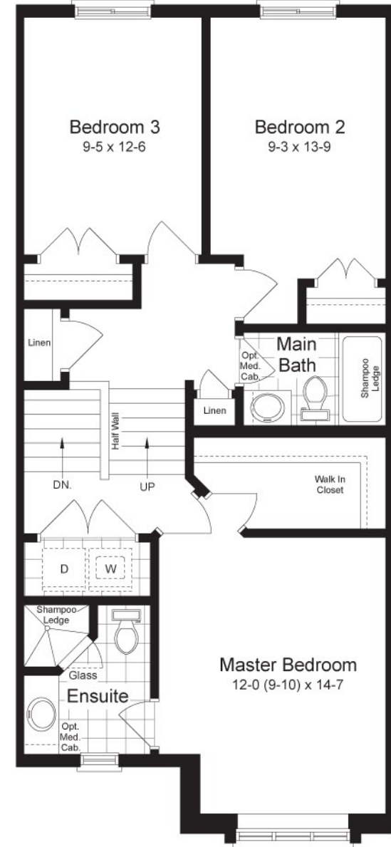
SECOND FLOORPLAN
